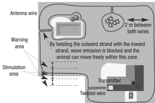
Diagram 3 – Sample installation
